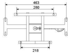
WSP-413 Lever for seat height adjustment
