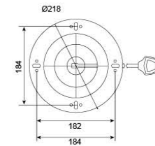
WSP-409 Lever for seat height adjustment
