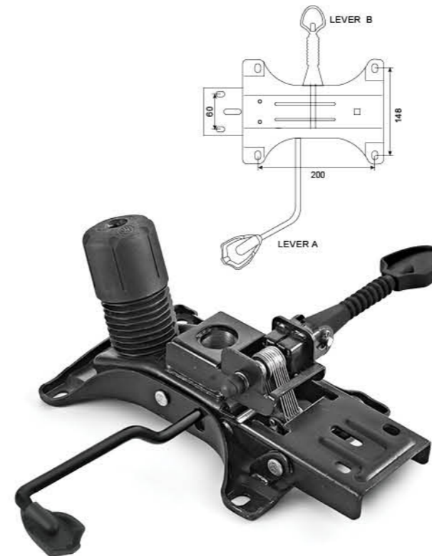
Lever A for seat height adjustment Lever B for locking at any angle
