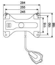
WSP-401 Lever for seat height adjustment
