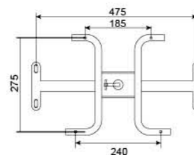
WSP-415 Lever for seat height adjustment
